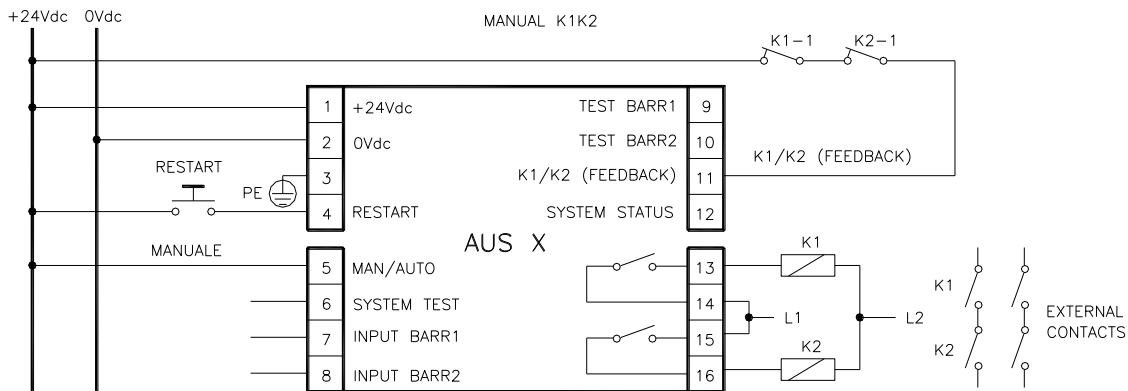
Figure 4 Manual functioning with K1K2 relays
