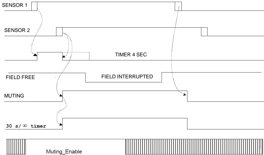
Figure 18 - Muting cycle
