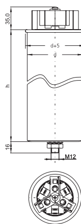
Capacitor with connection adapter ASS 2 d = 85 mm
