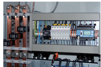
Fig.: Capacitor monitoring in a PFC system
