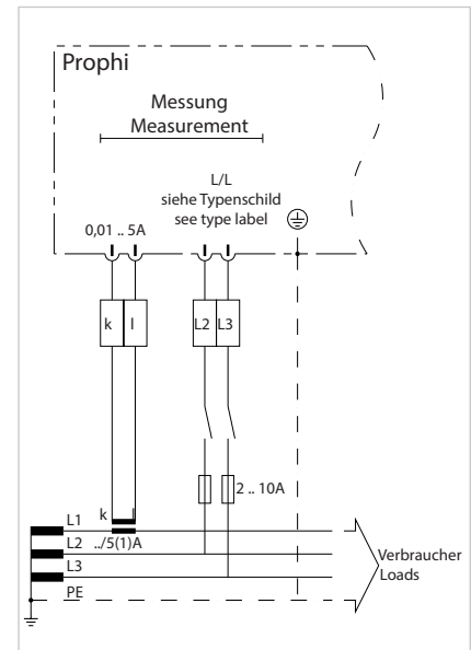
Fig.: Connection of measurement and auxiliary voltage between L2-L3 and the current measurement via current transformer
