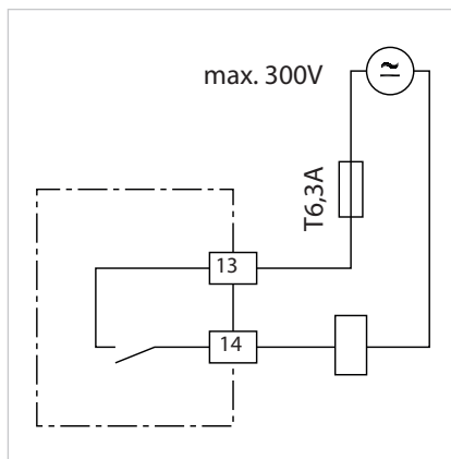
Fig.: Connection assignment, alarm output
