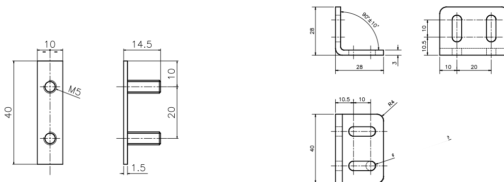
Figure 28 - FIE inserts and LE fastening brackets (provided)
