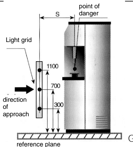
Figure 14 - Multibeam
