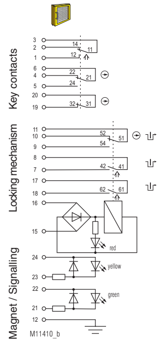
Fig. 2: Solenoid locking deactivated: Magnet released, optionally 1st key inserted, actuator and key inserted, Door closed
