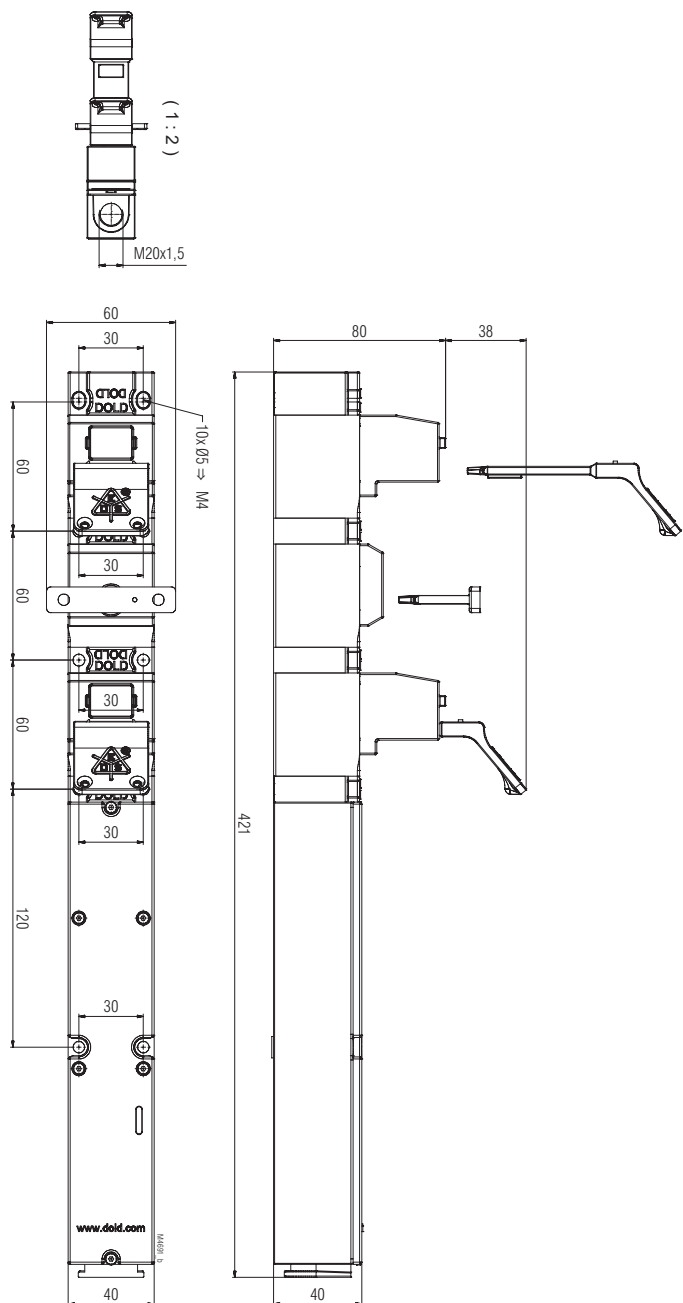
Illustrations: YRH10B01M Clearance tolerances \pm 2\%
