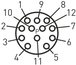
Contact diagram reset push-button
